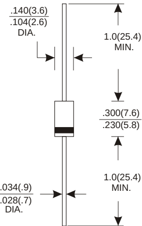
DO-15
