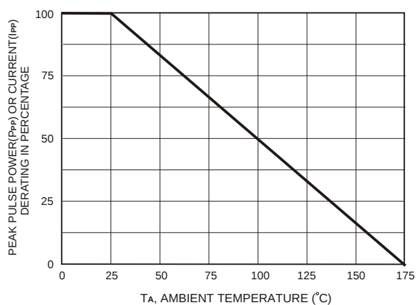
FIG.2-PULSE DERATING CURVE
