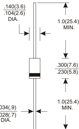
DO-15
